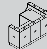
LIN39L 2444 / 1650 / 1105 6 3/8" / 65" / 43 1/2" LIN39P 2444 / 1650 / 1105 96 3/8" / 65" / 43 1/2"
