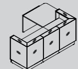
LIN41L 2744 / 1850 / 1105 96 3/8" / 80 3/4" / 43 1/2" LGC41P 2744 / 1850 / 1105 108 1/8" / 72 7/8" / 43 1/2"
